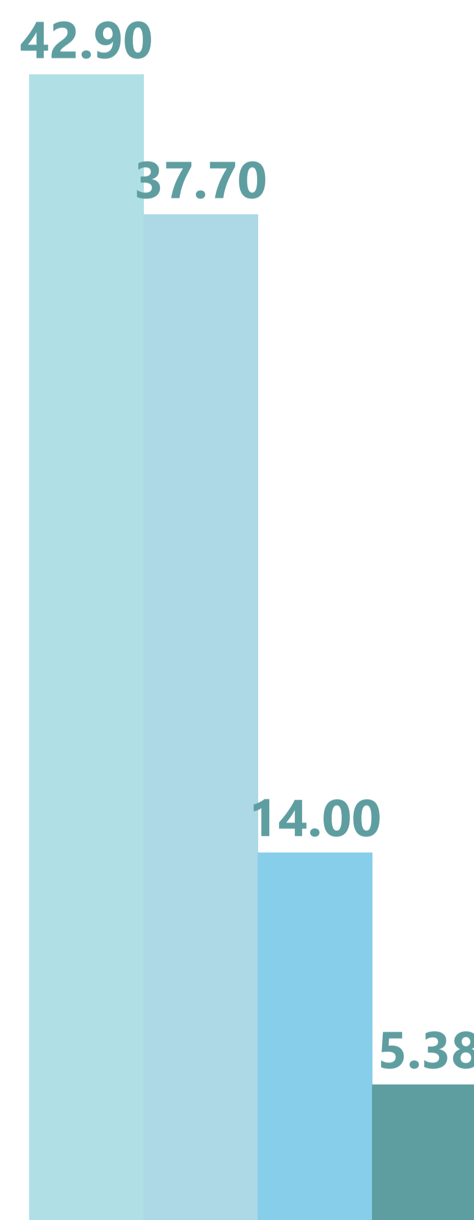
Stage*% Distribution
